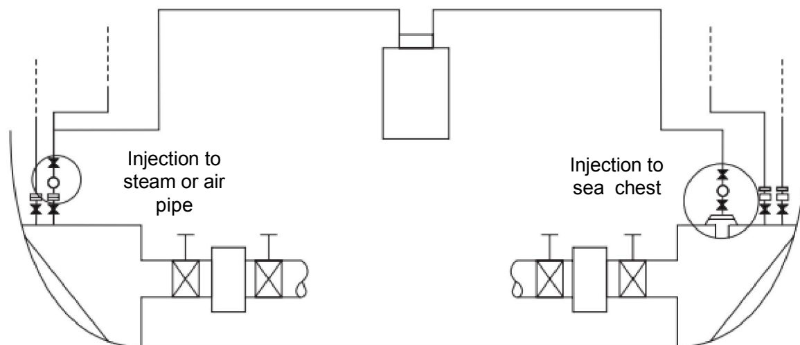
Sea Water Dosing Unit
