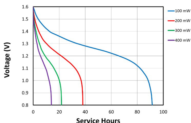
Constant Power
