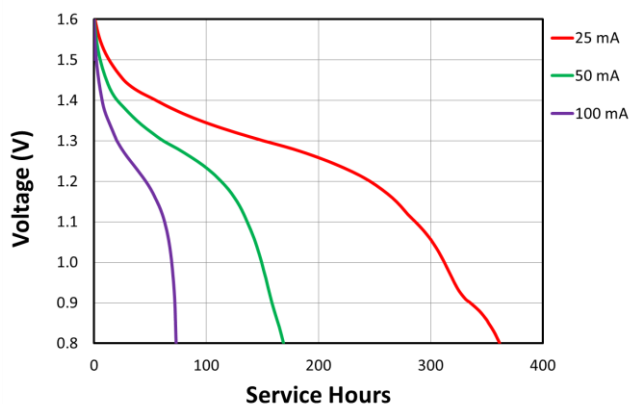
Constant Current
