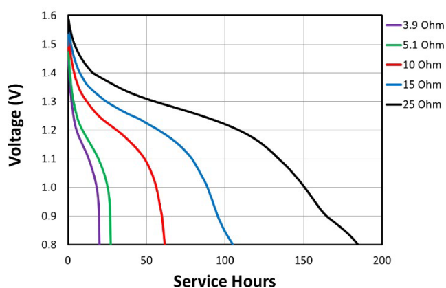
Constant Resistance
