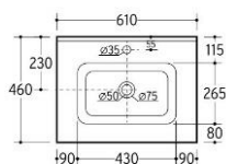
E-8092-60 Size: 610x460x175mm
