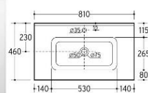
E-8092-80 Size: 810x460x175mm
