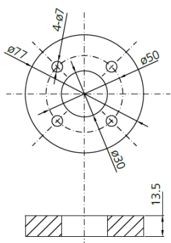
Passer for DN50 - DN80 Suitable for DN50 - DN80
