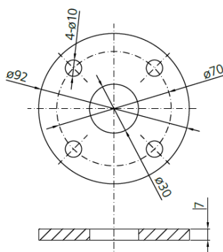
Passer for DN100 - DN150 Suitable for DN100 - DN150
