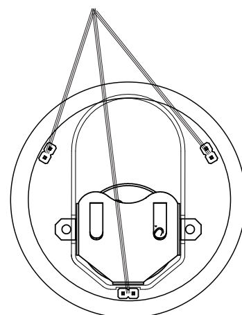
Fuktsensorer
