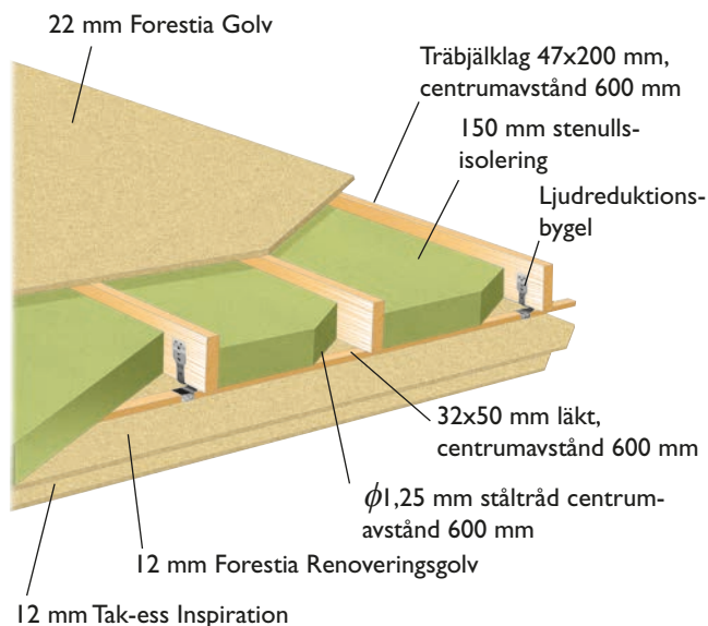
REI 60 (Sintef-NBL 25000.10/93.109, 250060/93.163)
