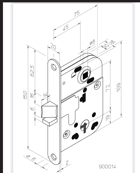
Lock case dimensions (mm)
