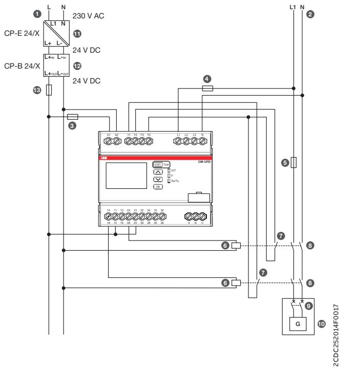
Example of single-phase application
