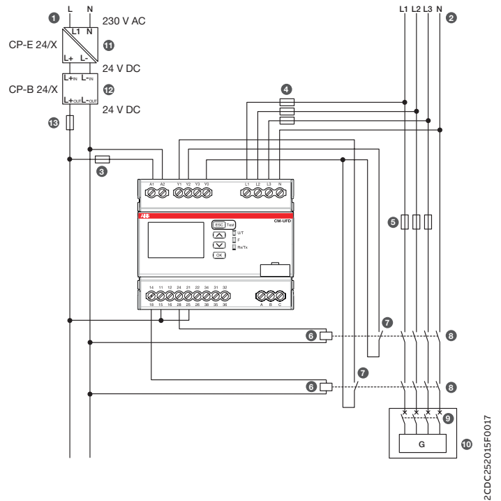
Example of three-phase application
