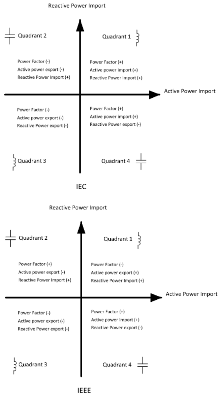
Figure 3-5 PF Convention
