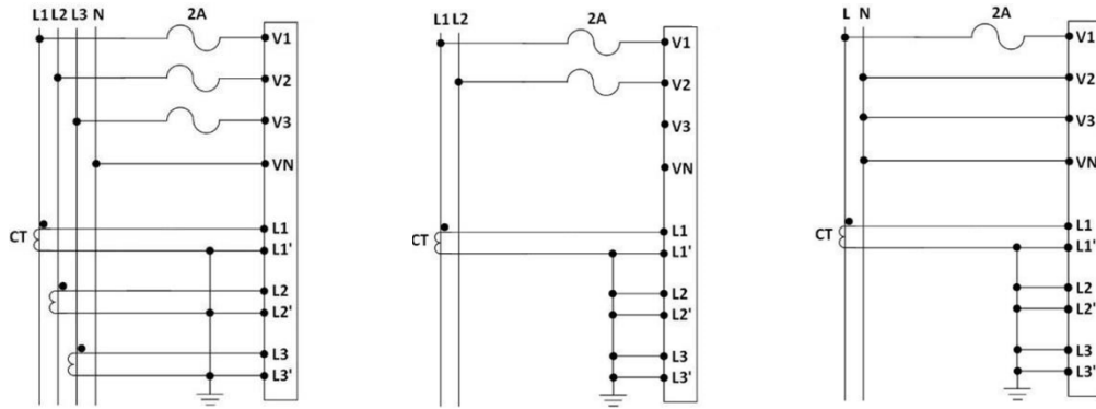
3P4W with 3CTs
