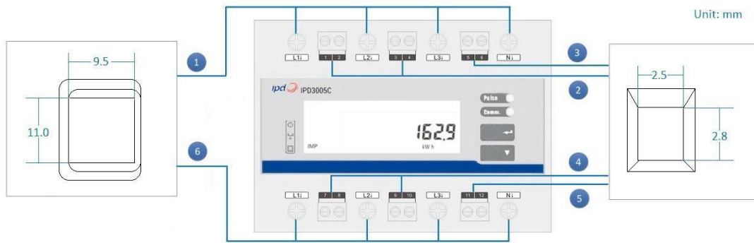
Figure 2-3 Terminal Dimensions
