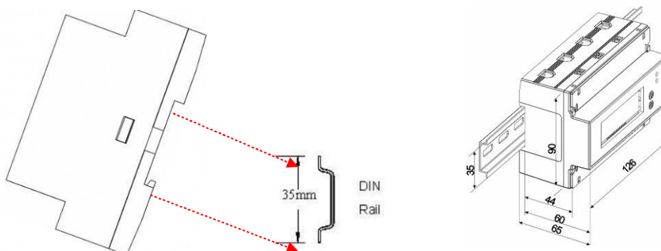
Figure 2-4 Installation
