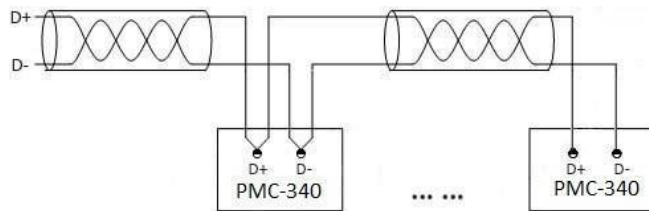
Figure 2-7 RS-485 Connections
