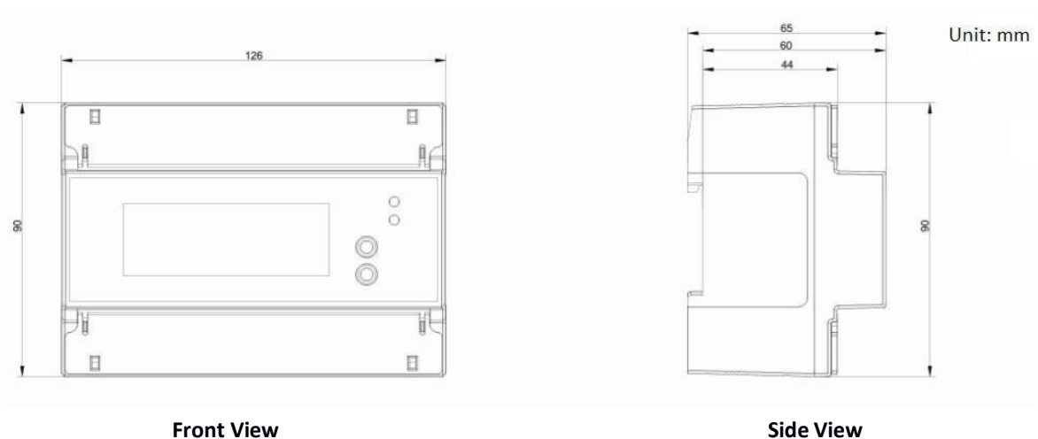
Figure 2-2 Dimensions
