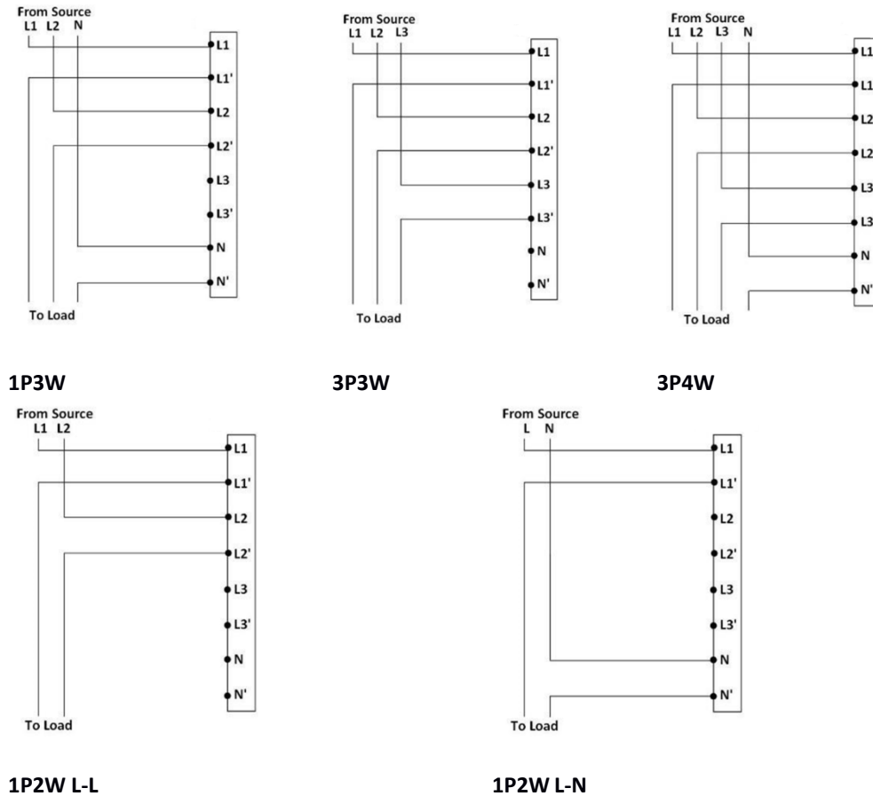
Figure 2-5 Direct Input connections
