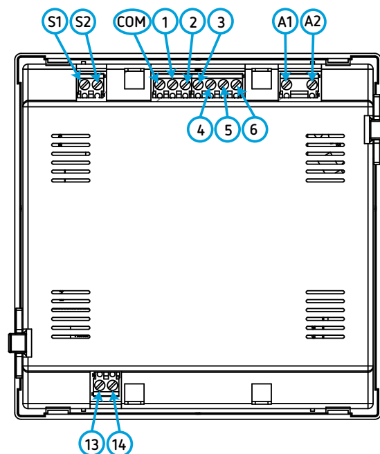
Figure 2: computer C6 Wi-Fi terminals
