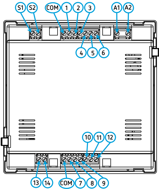
Figure 3: computer C12 Wi-Fi terminals
