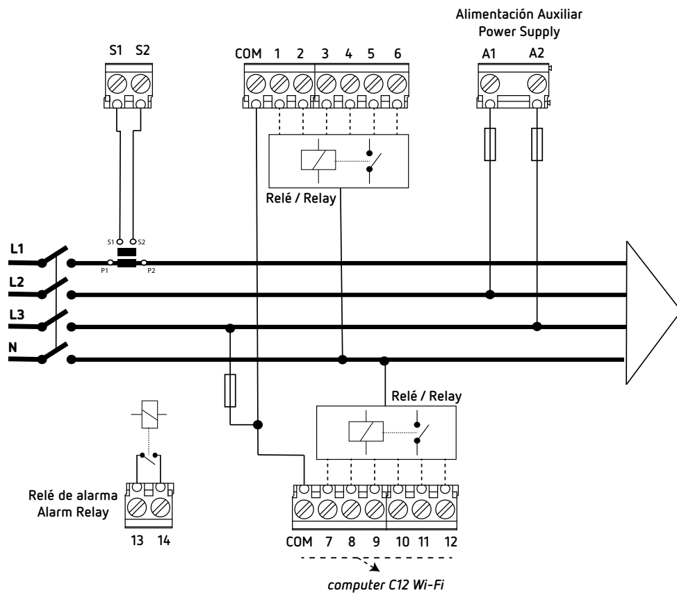
Figure 4: computer C Wi-Fi connection diagram.
