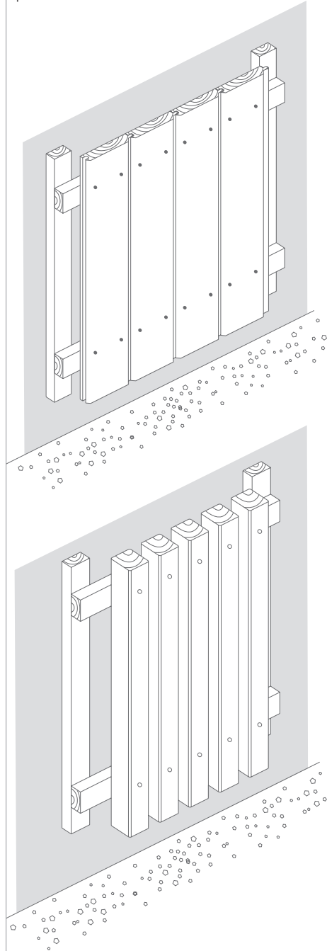
Benchmark by Thermory Thermo-ash cladding. Hidden installation with PaCS Clad (powered by Grad). Private house in USA. Designed by DIG:A
