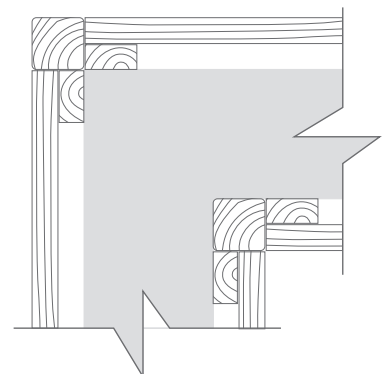
Use C4 42 x 42 mm profile.
