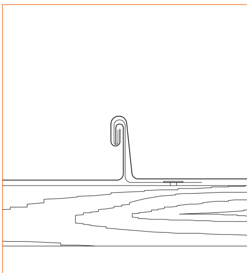
e) closing to the double standing seam
