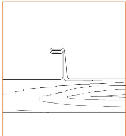
d) hand- or machine-made closing to angled standing seam
