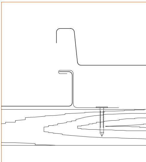
c) the following panel placing
