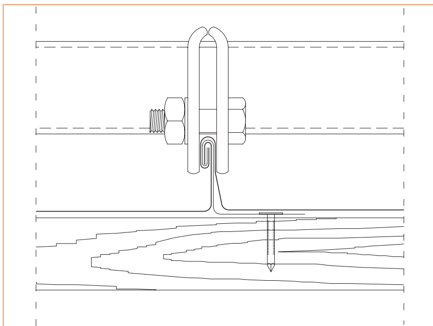
Drawing 8 The way of safety accessories fastening to the seam
