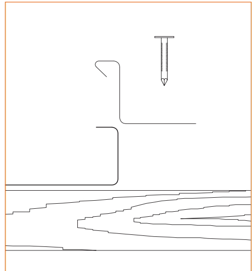
b) indirect fastening of the panel with the clip
