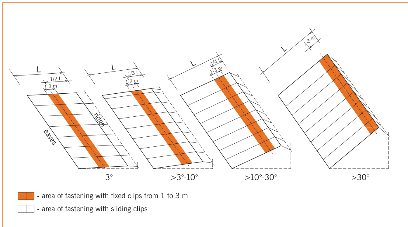
Drawing 7 Diagram of fixed clips placing depending on roof inclination
