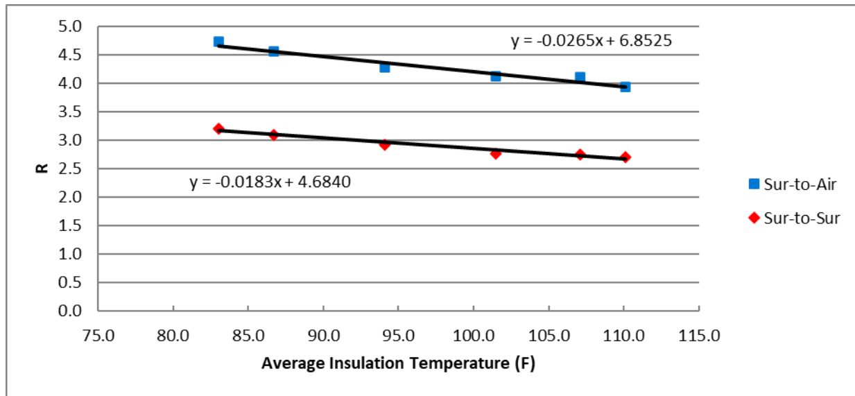
Figure 1. R-Value Of Duct Insulation Versus Average Insulation Temperature
